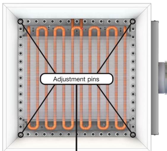
plastic pin 1
