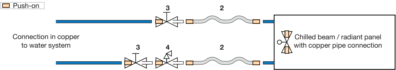
Picture 3. Connection to a 2-pipe unit - with integrated 2-way valve.
