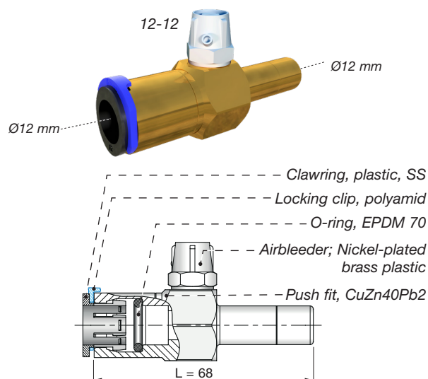
Picture 12. Section view of Air vent - Connector with airbleeder.
