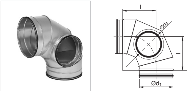
BFKCU 90°. cleaning bend
