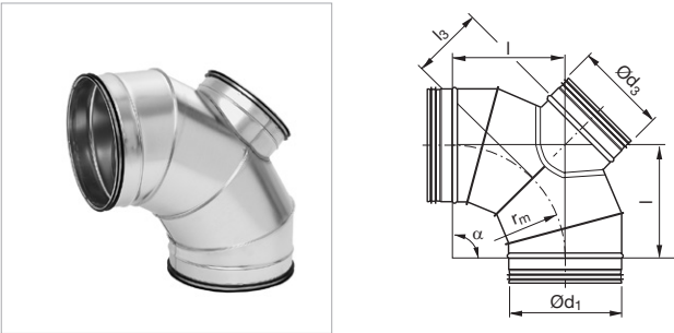
BFBKCU 90°. cleaning bend
