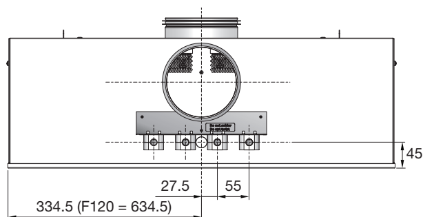
F-60: 2-pipe battery (standard).
